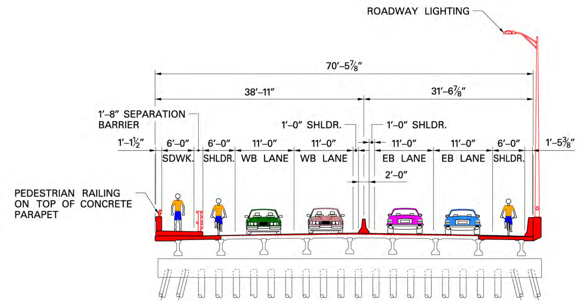
PROPOSED TRESTLE BRIDGES (LOOKING EAST)
