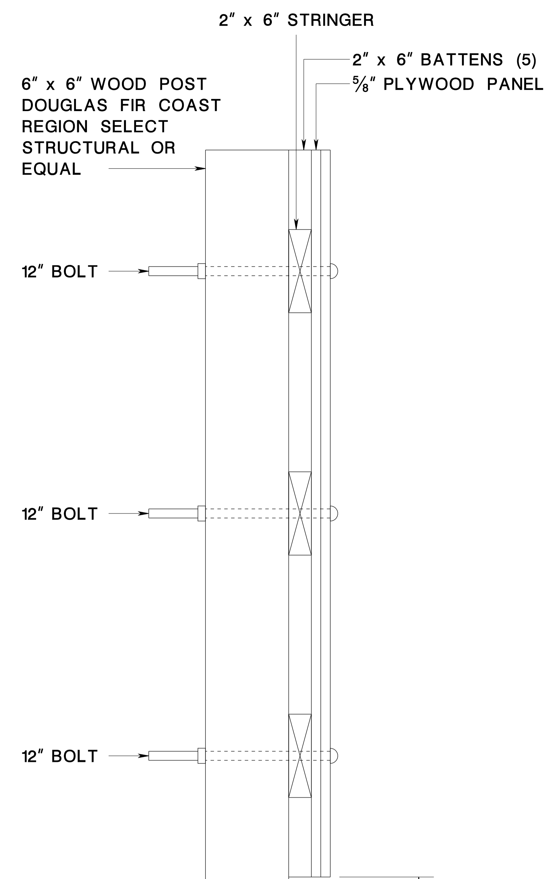
DETAIL OF BATTEN AT PLYWOOD JOINTS
