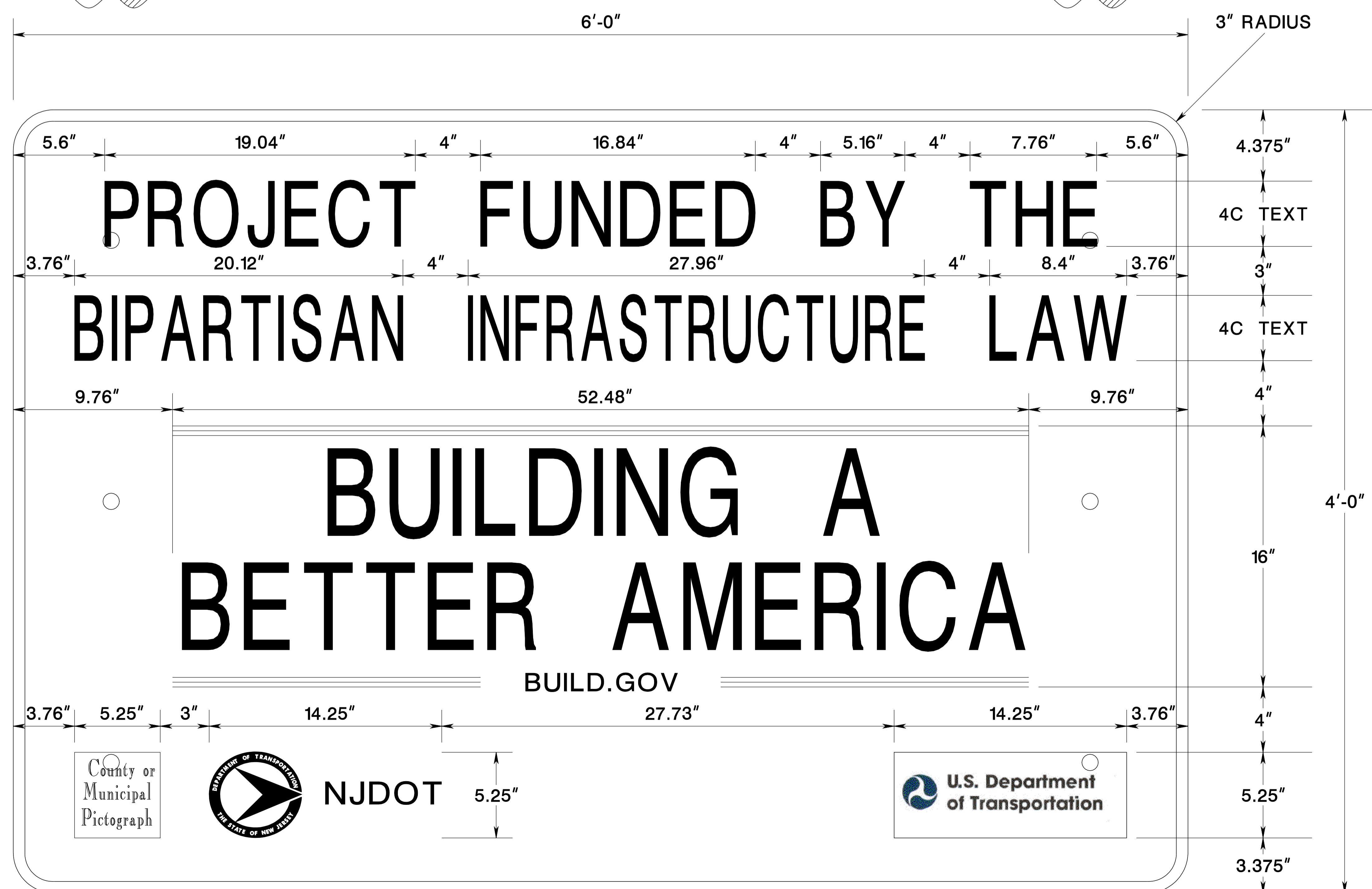
DETAIL OF TEXT ALIGNMENT
