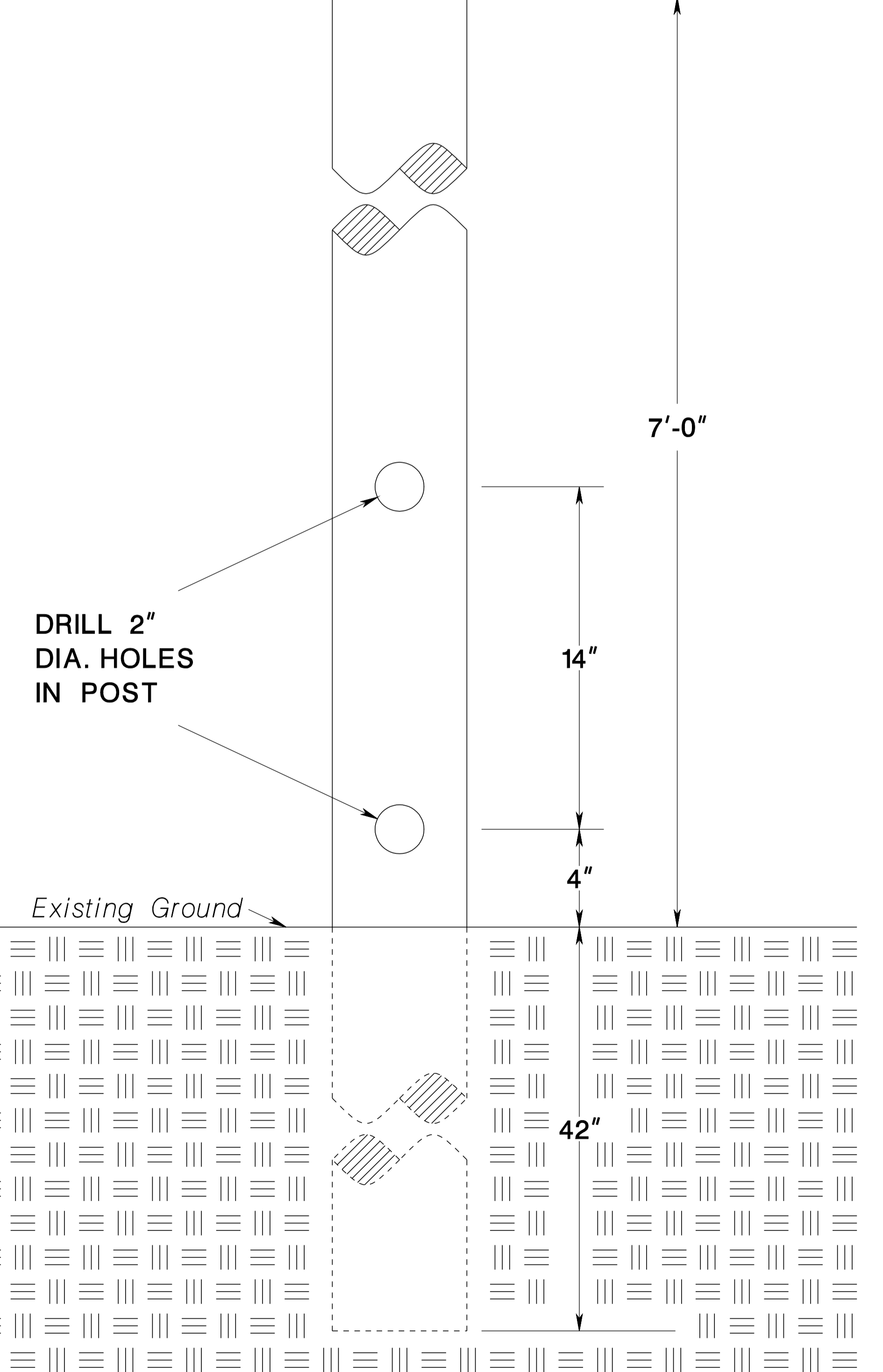
SIDE VIEW OF SIGN STRUCTURE
